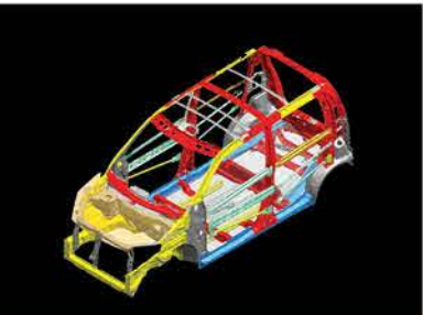
Energy Absorbing Structure for Safer Drive
