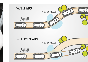
NEW-GEN ABS WITH MOTOR SPEED REGULATION SYSTEM
